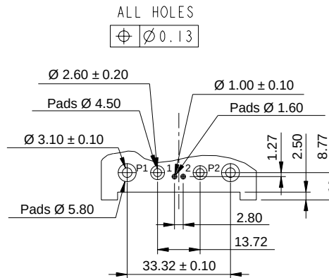
PCB drill & recommended pad details (PCB thickness - 1.6 mm)
