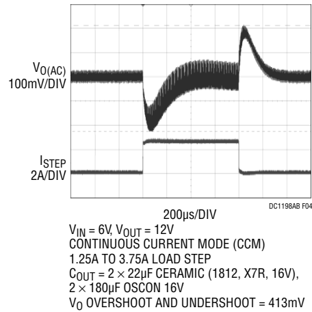
Figure 4. Measured Load Transient Response (2.5A Step, 25% to 75%)
