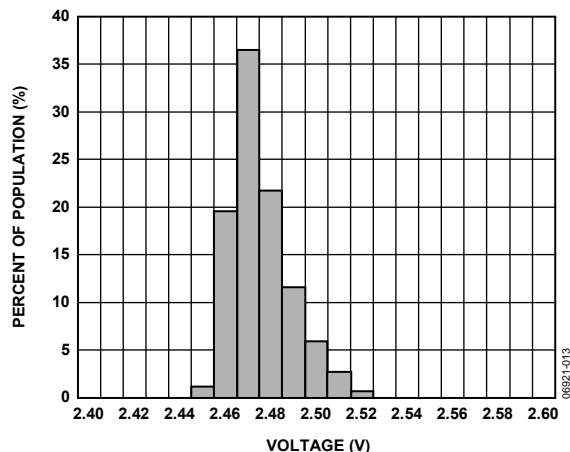
Figure 13. V TEMP Output at 25°C (V RATIO = 5 V)
