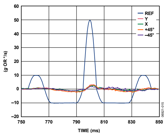
Figure 15. g and g × g Sensitivity for a 50 g, 10 ms Pulse
