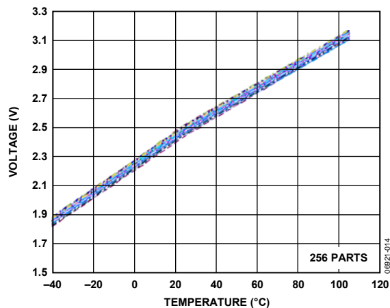
Figure 14. V TEMP Output over Temperature (V RATIO = 5 V)
