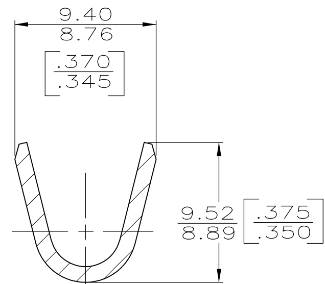
SECTION B-B
