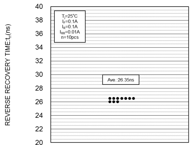
t_{tr} DISPERSION MAP
