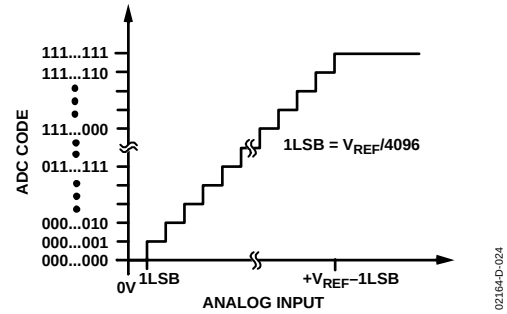
Figure 24. Transfer Characteristic
