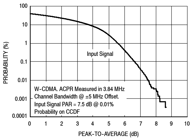
Figure 13. CCDF W-CDMA IQ Magnitude Clipping, Single-Carrier Test Signal
