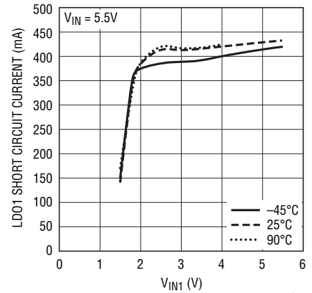
LD01 Short Circuit Current vs V_{IN1}
