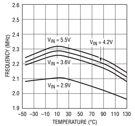
Buck Oscillator Frequency vs Temperature
