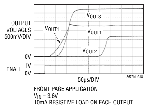
Startup Transient
