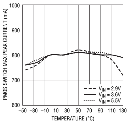
PMOS Switch Maximum Peak Current
