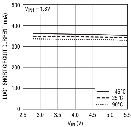
LD01 Short Circuit Current vs V_{IN}
