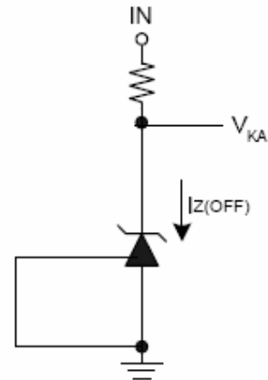
Figure 3. Off-state Current
