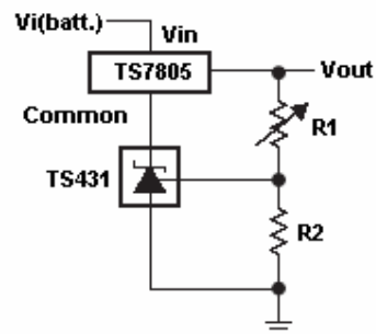
V_{out} = V_{ref} * (1 + R1 / R2) minimum V_{out} = V_{ref} + 5V
