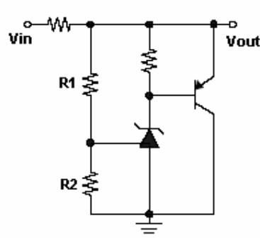
V_{out} = V_{ref} * (1 + R1 / R2)
