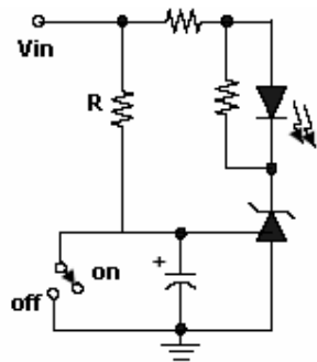
Delay = RC \ln (V_{in} / (V_{in} - V_{ref}))
