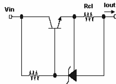
I_{out} = V_{ref} / R_{cl}
