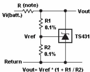
V_{out} = V_{ref} * (1 + R1 / R2)
