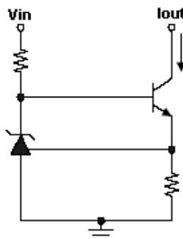
I_{out} = V_{ref} / R_s
