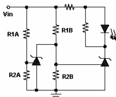
LED on when low limit < Vin < high limit low limit = V_{ref} (1 + R1B / R2B) high limit = V_{ref} (1 + R1A / R2A)
