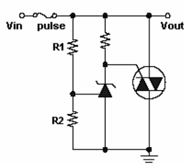
Limit = V_{ref} * (1 + R1 / R2)
