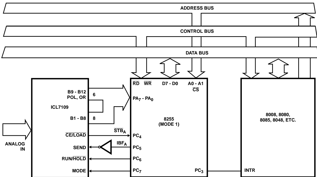
FIGURE 19. HANDSHAKE INTERFACE - ICL7109 TO 8048, 80/85
