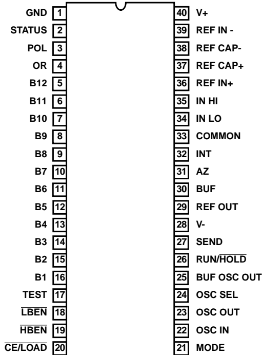
ICL7109 (CERDIP, PDIP, SBDIP) TOP VIEW
