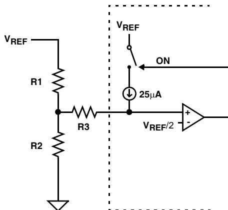
FIGURE 11. OTS HYSTERESIS
