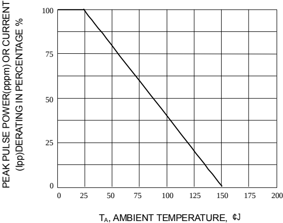
Fig. 2-PULSE DERATING CURVE
