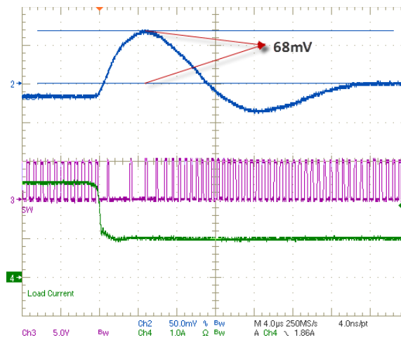
CH2: VOUT, CH3: SW, CH4: Load Current Figure 11. VOUT = 1.8V, L = 4.9µH
