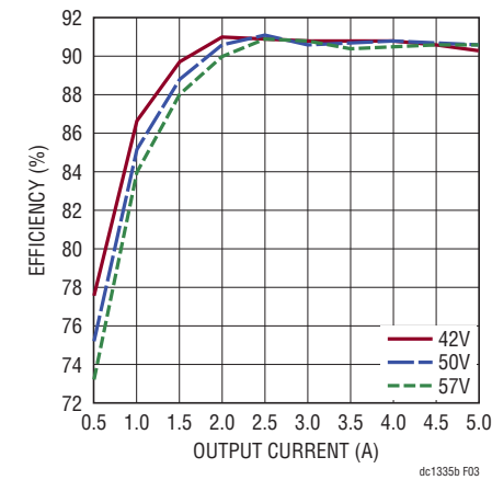
Figure 3. Efficiency (Not Including Diode Bridge)
