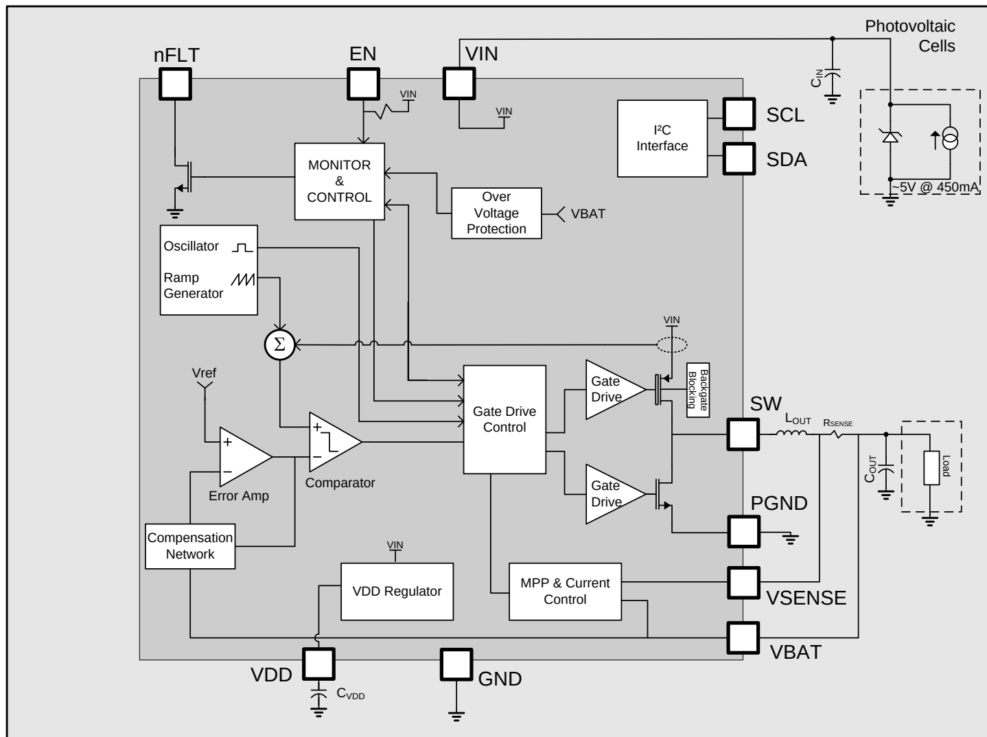
Figure 2: TS52002 Block Diagram
