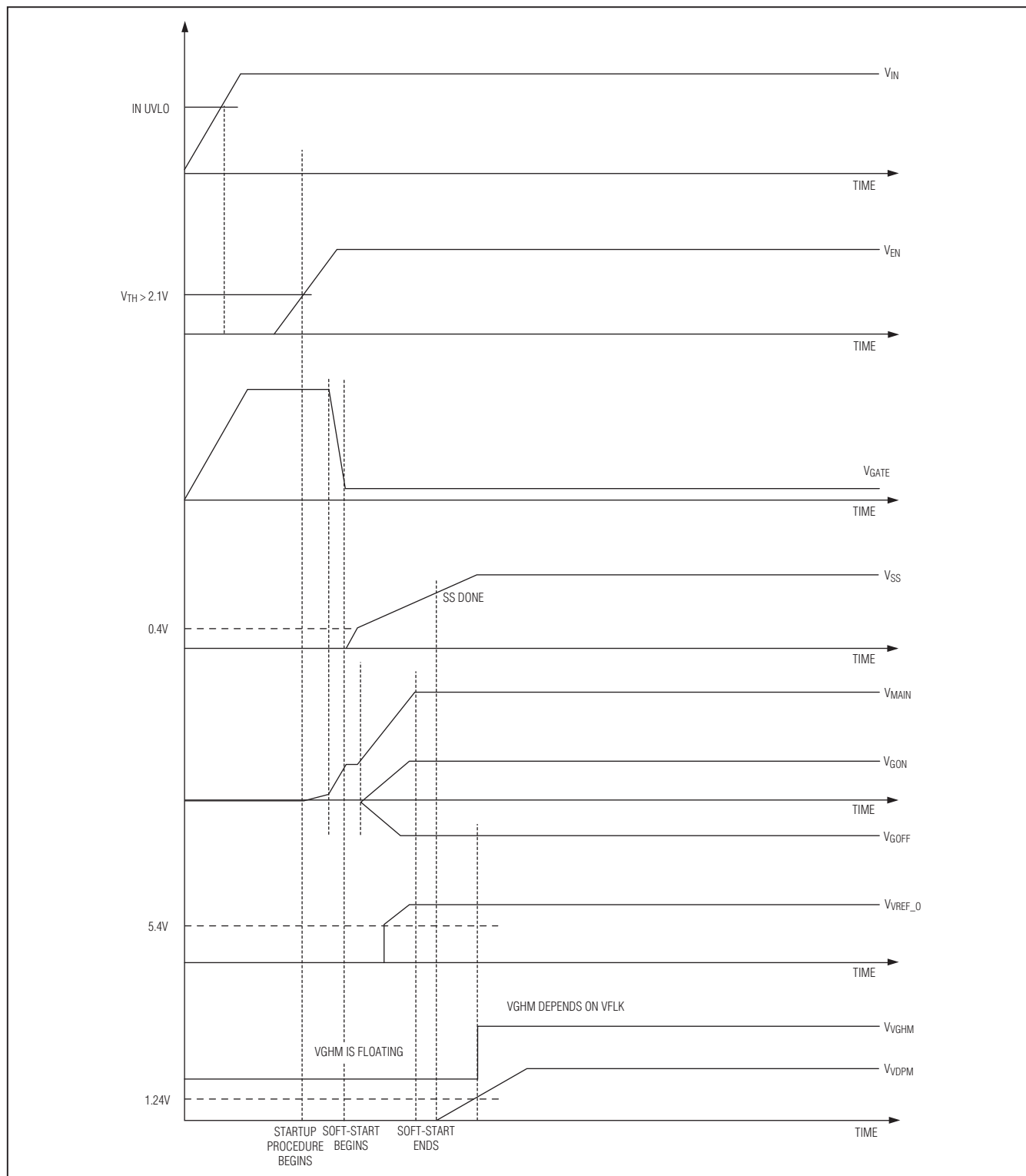
Figure 4. Power-Up Sequence
