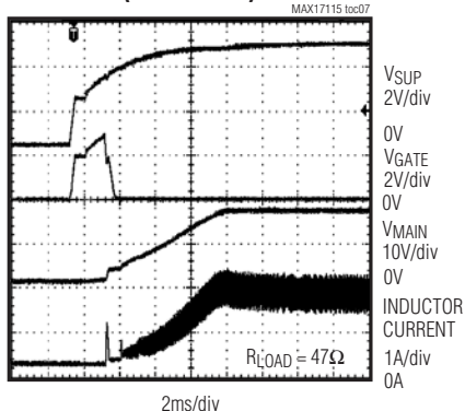
STEP-UP REGULATOR SOFT-START (HEAVY LOAD)
