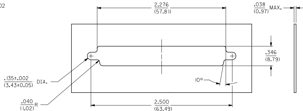
PANEL CUT-OUT DIMENSIONS
