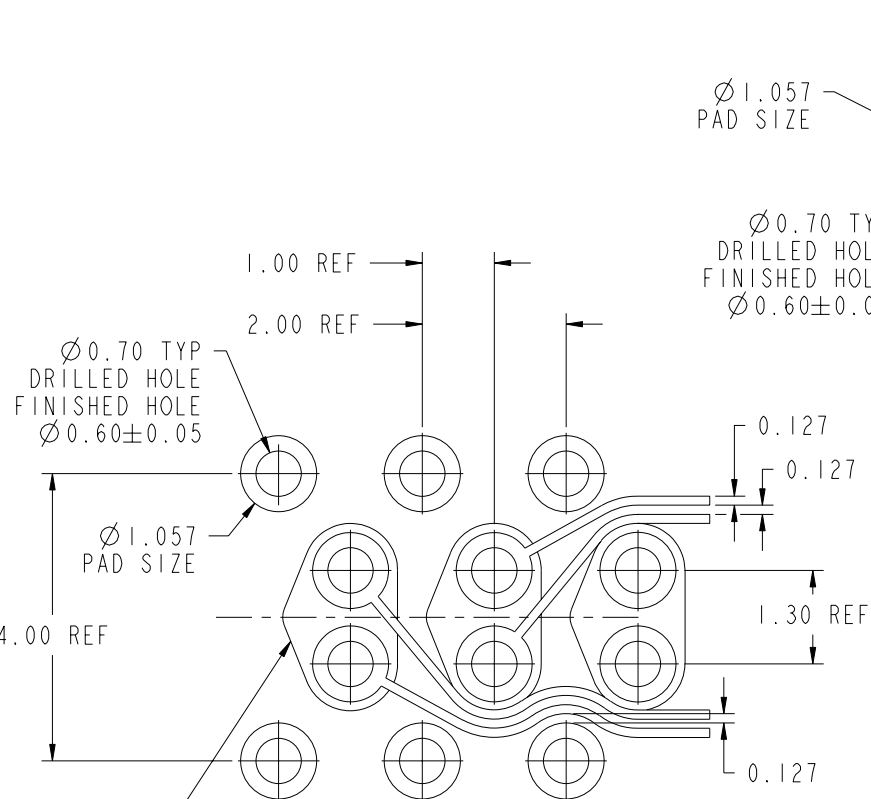
OPTION A (EDGE COUPLED) DIFFERENTIAL PCB TRACE LAYOUT
