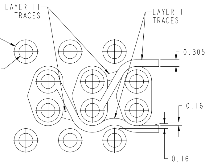
OPTION B (BROADSIDE COUPLED) DIFFERENTIAL PCB TRACE LAYOUT
