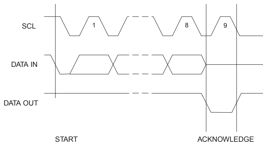
Figure 4-5. Output Acknowledge
