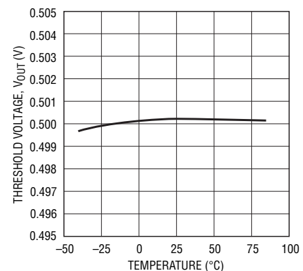
Input Threshold Voltage vs Temperature
