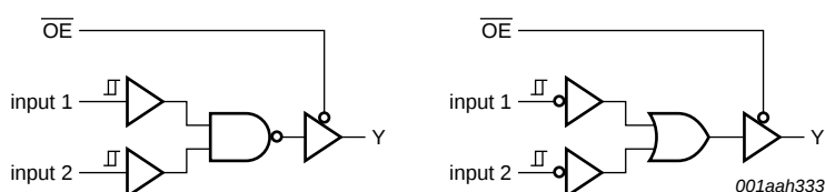
Fig 13. 3-state NAND/OR function
