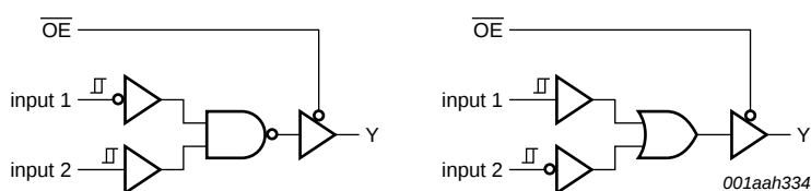
Fig 14. 3-state NAND/OR function
