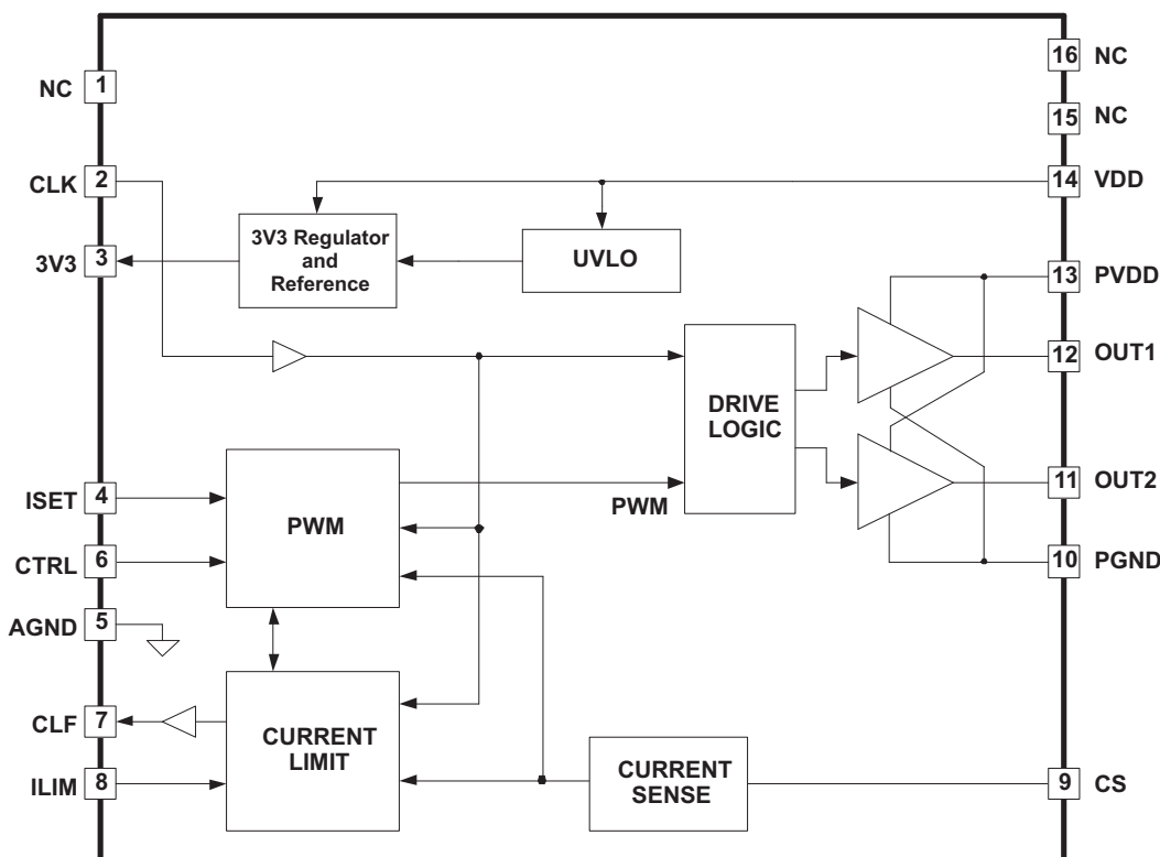
Figure 4. UCD8220
