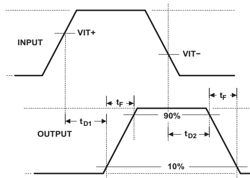
Figure 3. Timing Diagram
