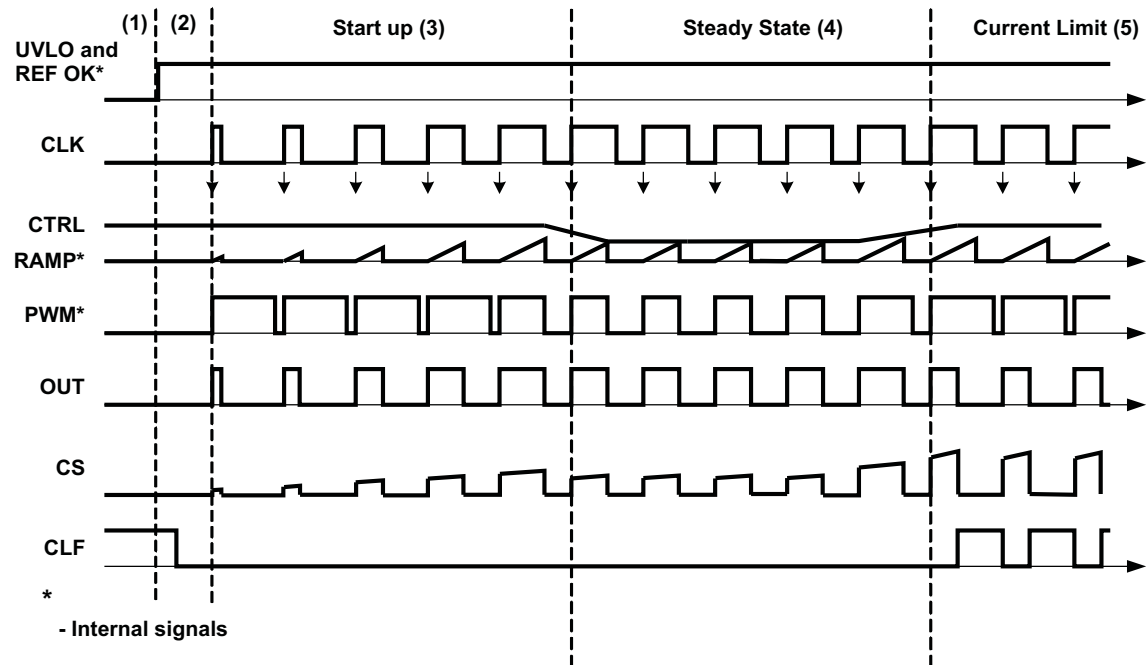
Figure 30. UCD8220 Timing and Circuit Operation Diagram
