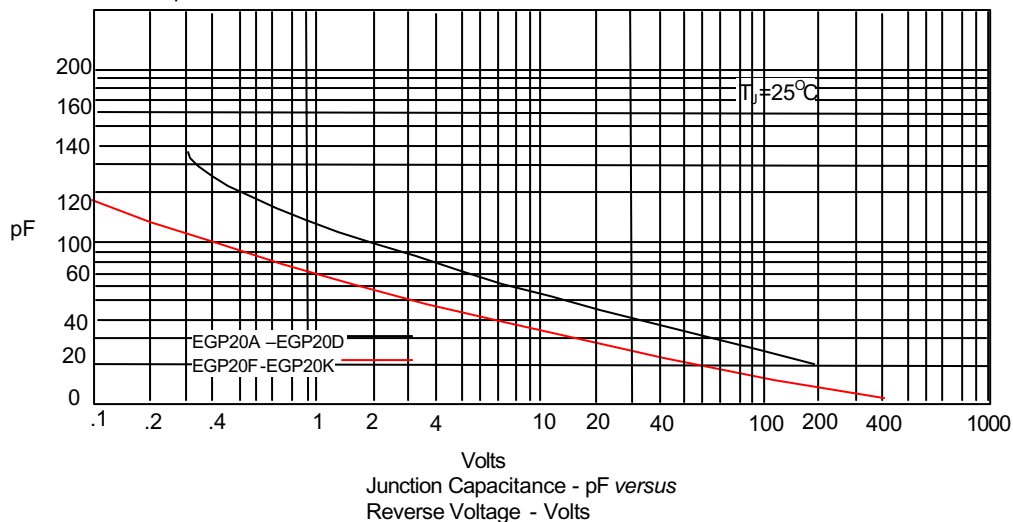
Figure 3 Junction Capacitance
