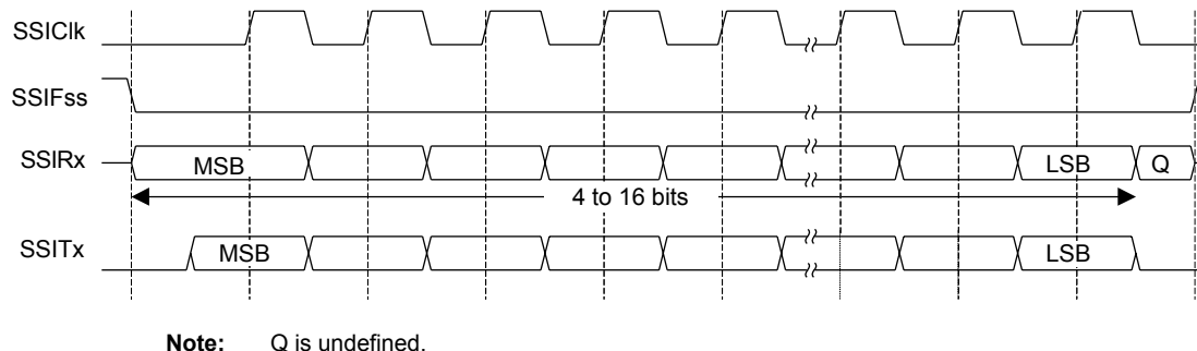
Figure 13-5. Freescale SPI Format (Continuous Transfer) with SPO=0 and SPH=0
