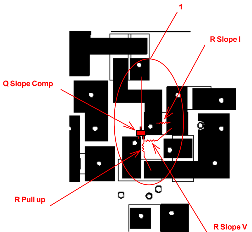
Board Layout Bottom
