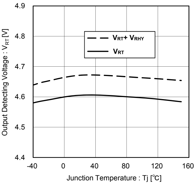
Figure 14. Output Detecting Voltage vs Junction Temperature
