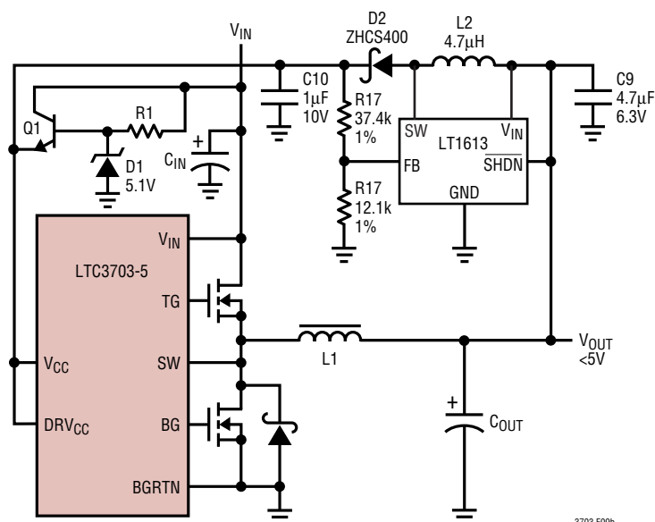
Figure 9b. V_{CC} Generated from V_{OUT} < 5V
