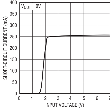
Current Limit
