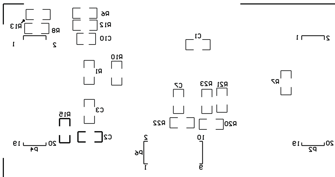
Figure 7. Bottom Silkscreen
