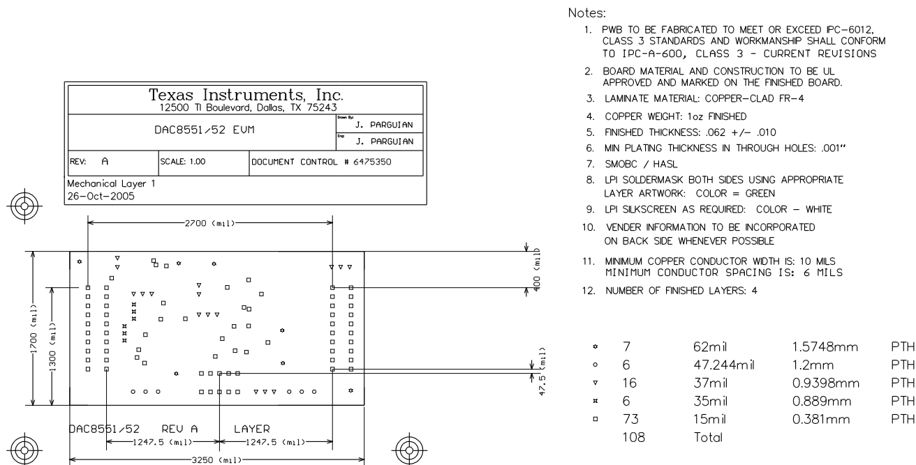
Figure 8. Drill Drawing
