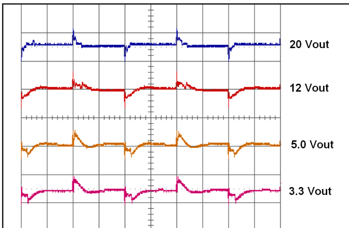
Figure 11: Output voltage response for 3.3V, 5V, 12V, 20V units to step-change in load current (50-75-50% of Iout max; di/dt=0.1A/µs). Load cap: 100µF, 100mΩ ESR tant, Ch 1-4: Vout (1V/div);(5ms/div).
