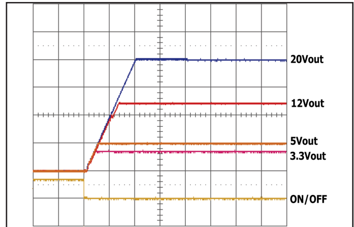
Figure 8: Turn-on transient at full load (resistive load) (50ms/div). ON/OFF input (5V/div) Ch 1-4: Vout (5V/div)
