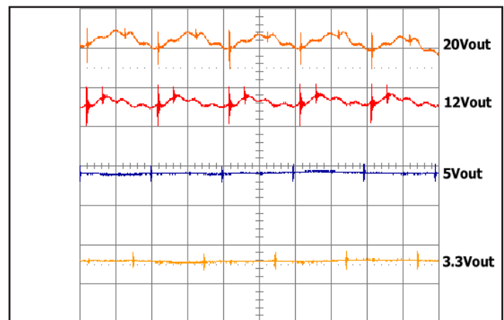
Figure 6: Output Voltage Ripple at 10V input voltage and rated load current (50mV/div). Zero load capacitance. Bandwidth: 20MHz. (See Fig 4)
