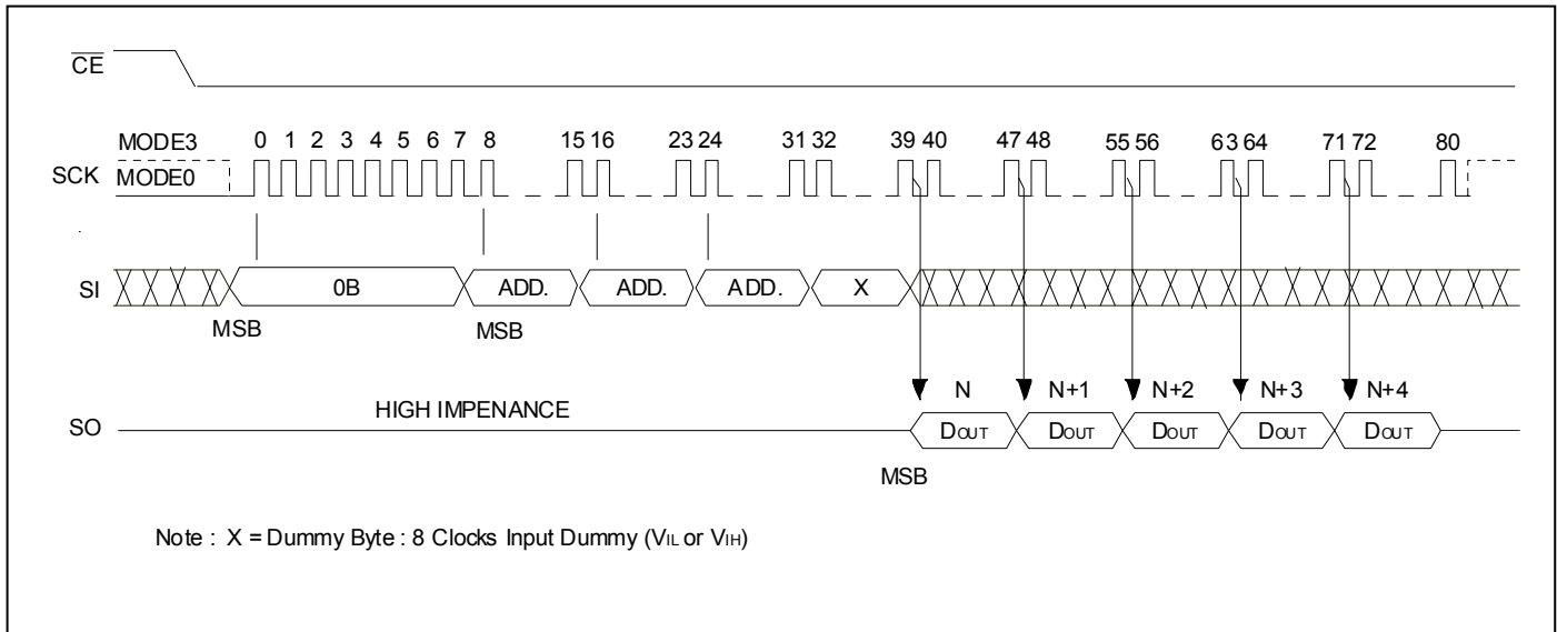
Figure 3 : HIGH-SPEED-READ SEQUENCE
