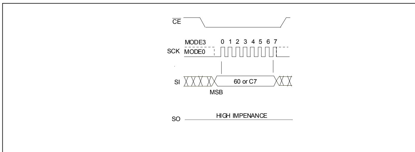
FIGURE 11 : CHIP-ERASE SEQUENCE
