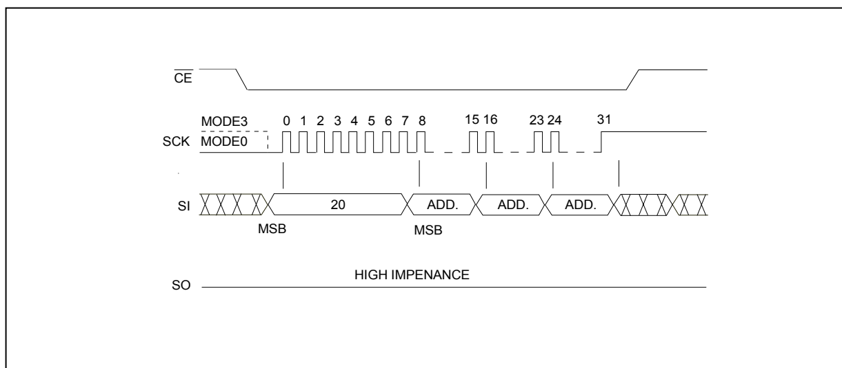
FIGURE 10 : SEQUENCE-ERASE SEQUENCE
