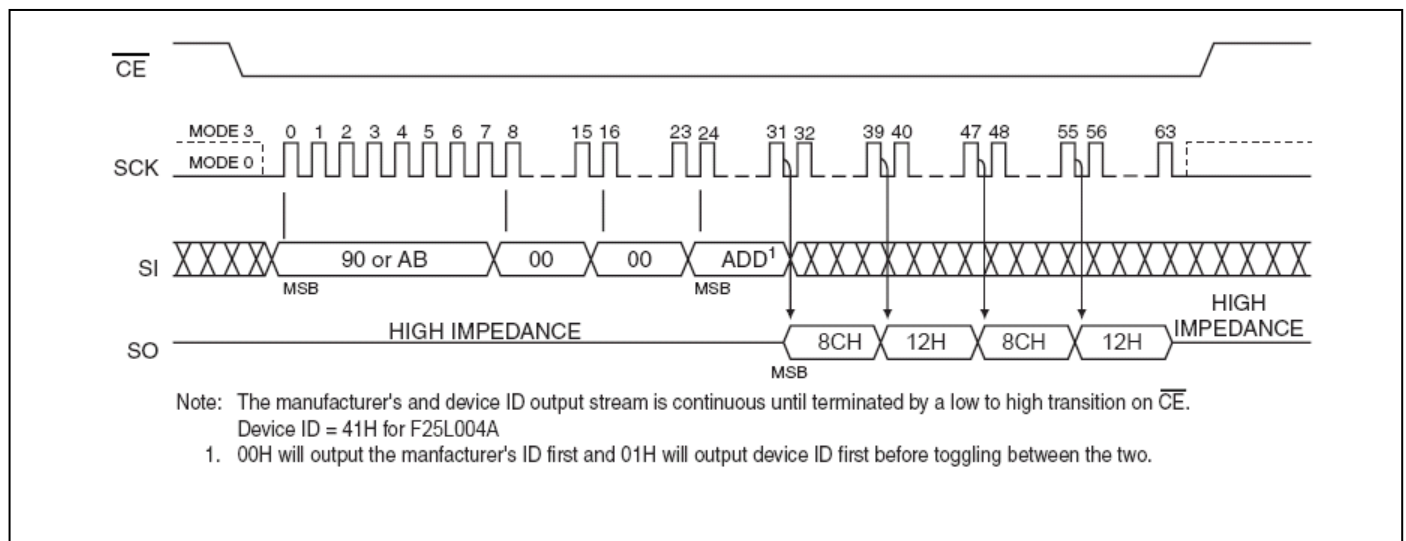
Figure 18 : Read-Electronic-Signature
