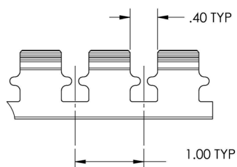
SLOTTED WALL DUCT TYPE "SL2X1"
