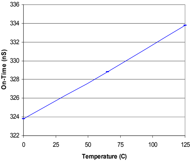
Figure 3. On-Time Variation in DCM: VIN = 12V, VOUT = 1.1V, RFF = 180kOhm
