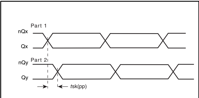
Part-to-Part Skew
