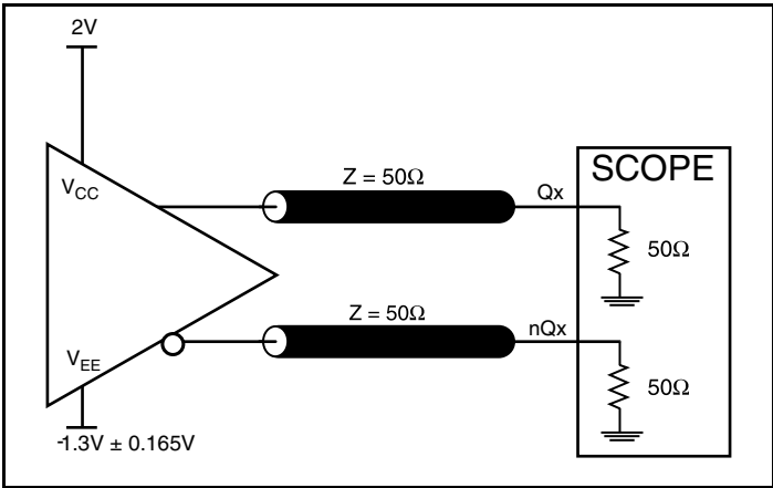
3.3V Output Load Test Circuit
