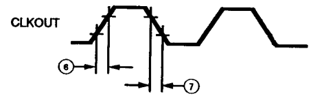
(b) CLKOUT Timing
