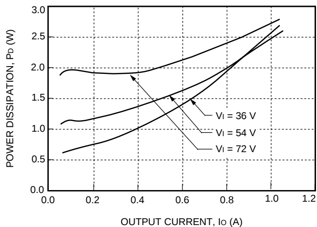
Figure 18. 12 V Output Power Dissipation vs. Output Current
