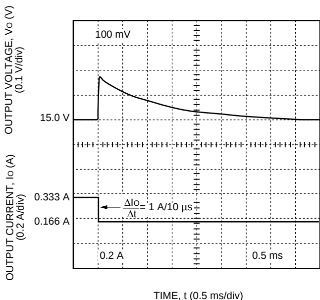
Figure 6. Typical DW025-Series 15 V Output Voltage Response to a Step Load Change from 50% to 25% of I_{o,max} at V_i = V_{i,nom} and T_A = 25^\circ\text{C}
