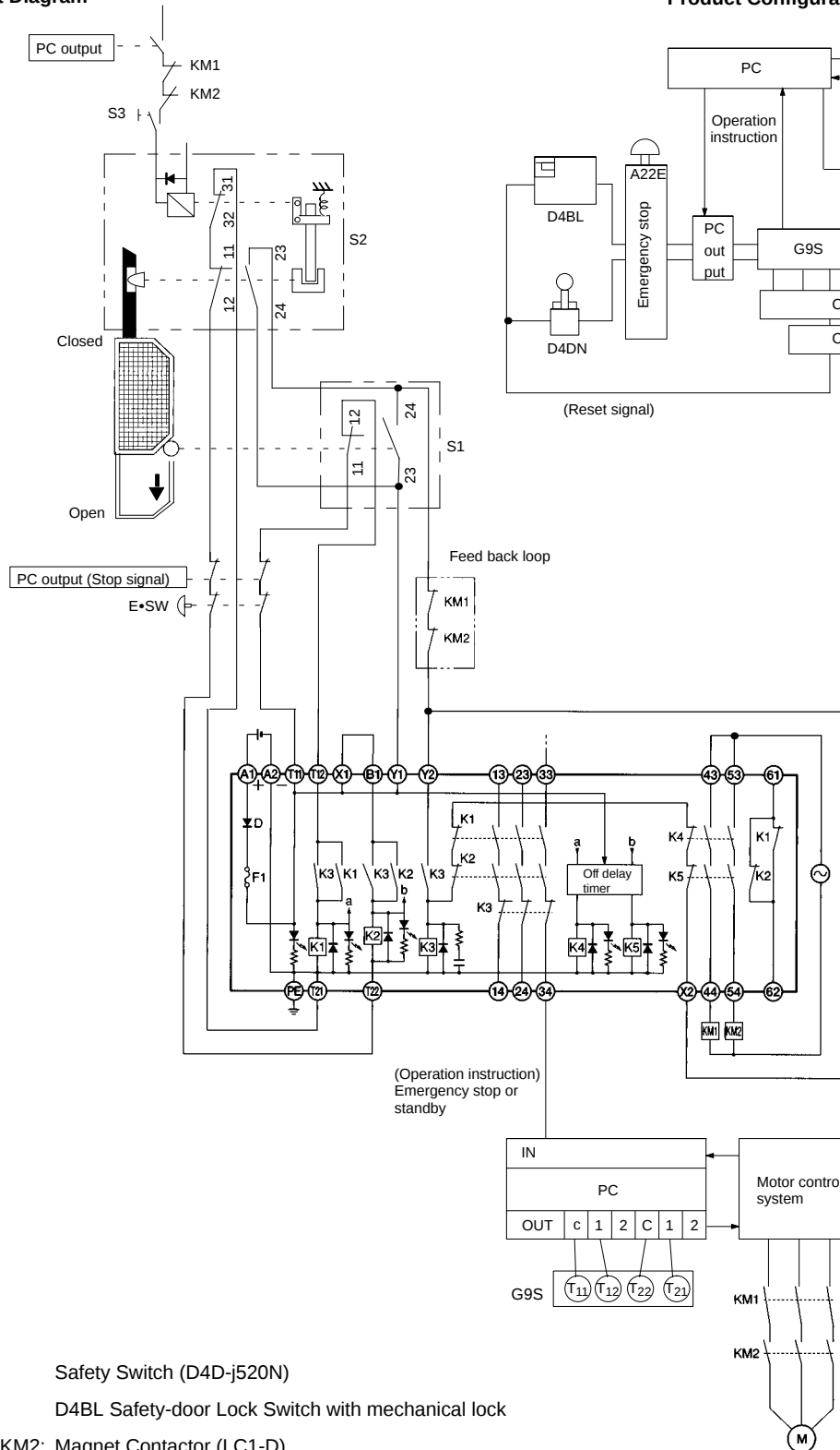
Circuit Diagram
