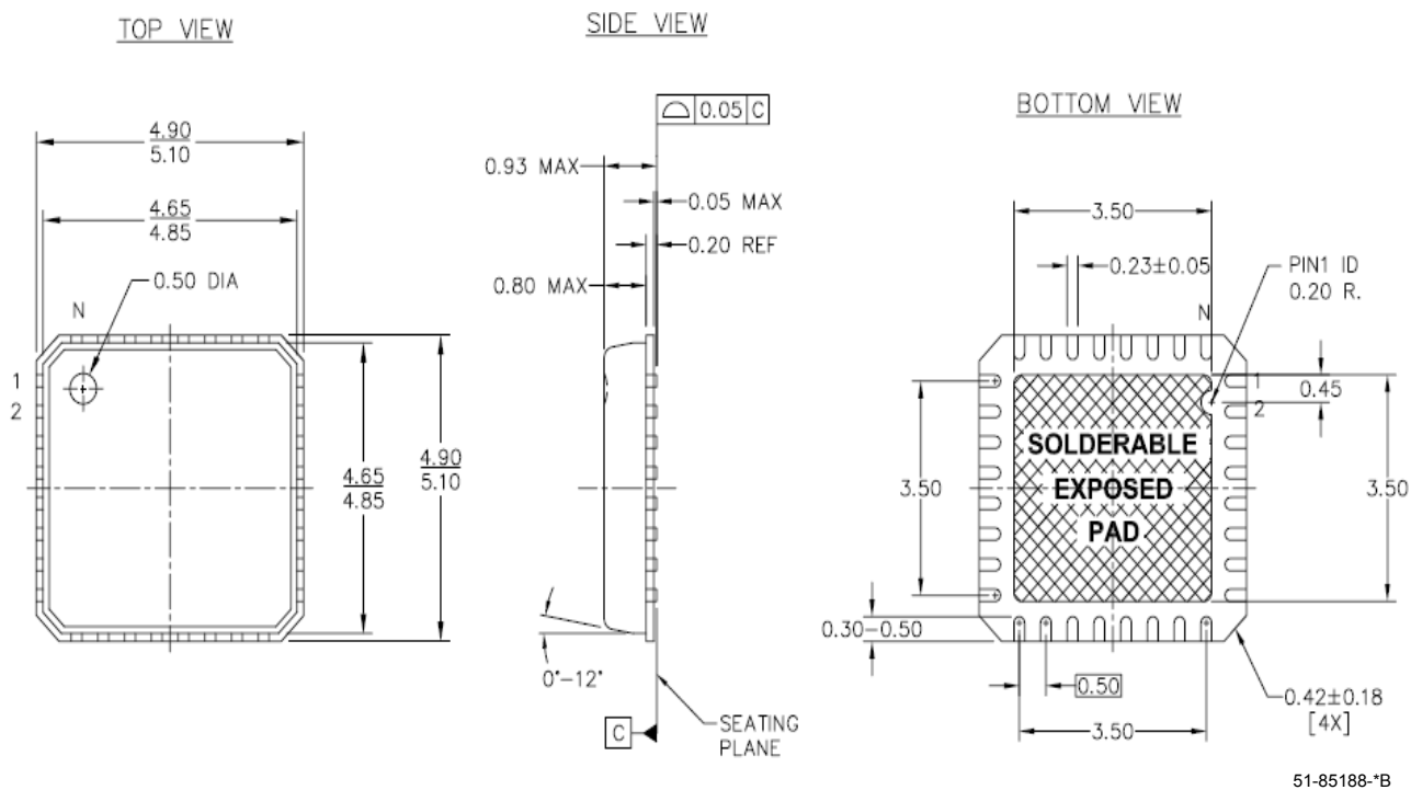
Figure 31-8. 32-Pin Sawn QFN Package
