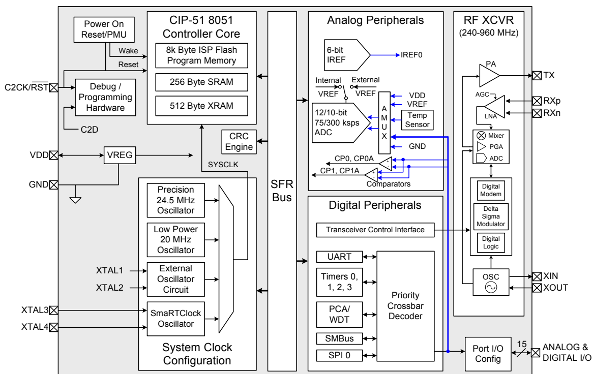
Figure 1.4. Si1013 Block Diagram
