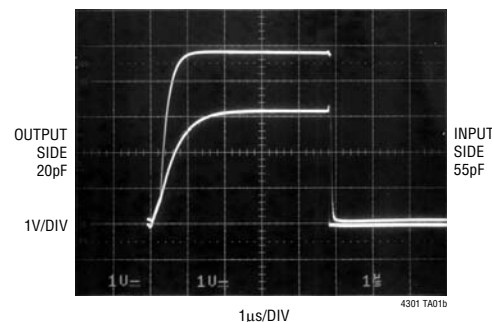
Input-Output Connection
