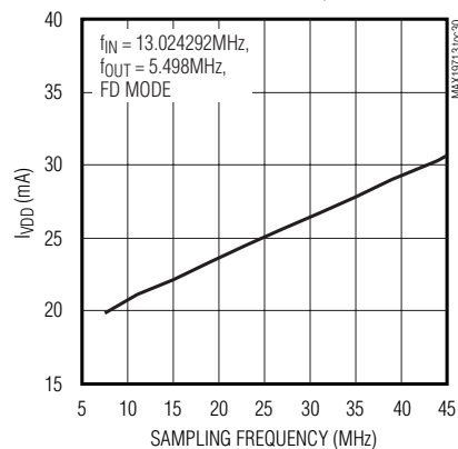
SUPPLY CURRENT vs. SAMPLING FREQUENCY
