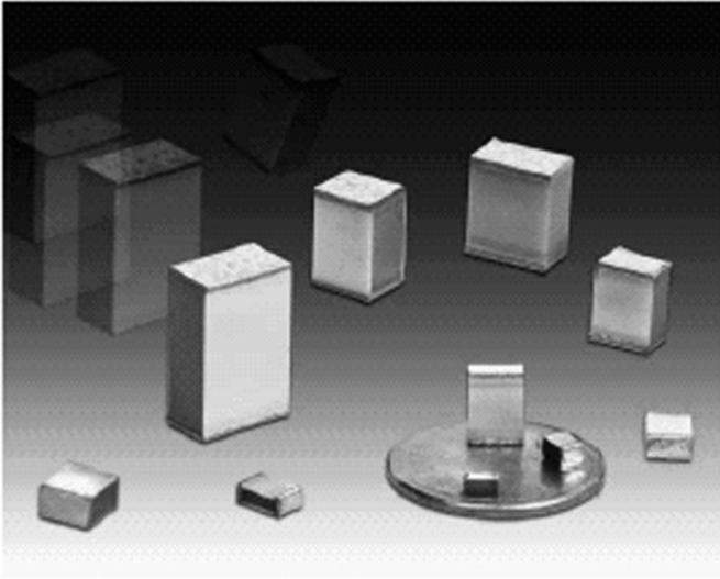
Type FCN SMT capacitors are the general purpose line of CDE's surface mount product offerings. They range in capacitance from .001 \mu\text{F} to 1.0 \mu\text{F} , and they are available in voltage ratings up to 400 Vdc.
