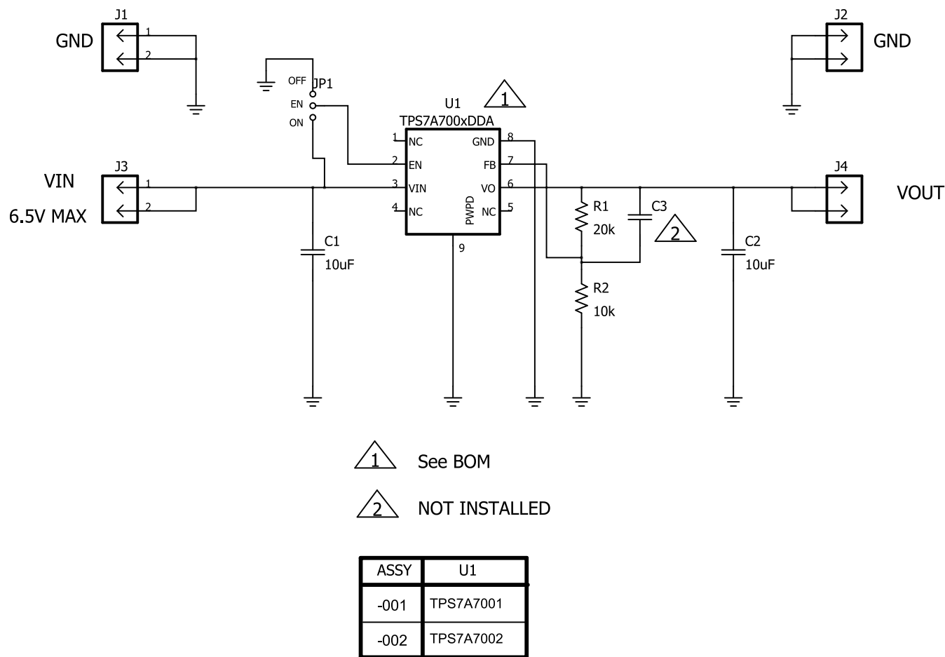
Figure 6. TPS7A7002EVM-065 Schematic
