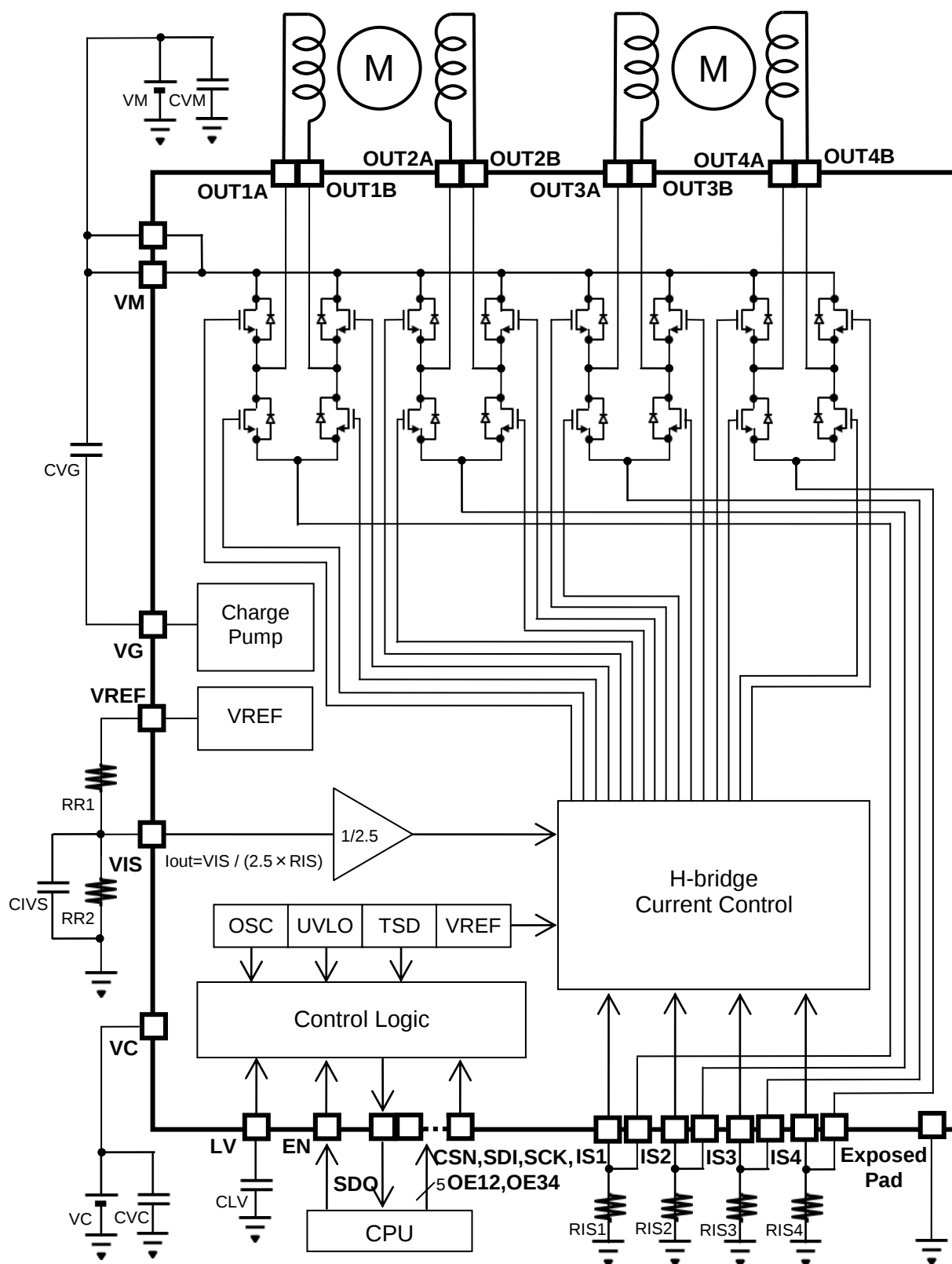
Figure 1. Block Diagram
