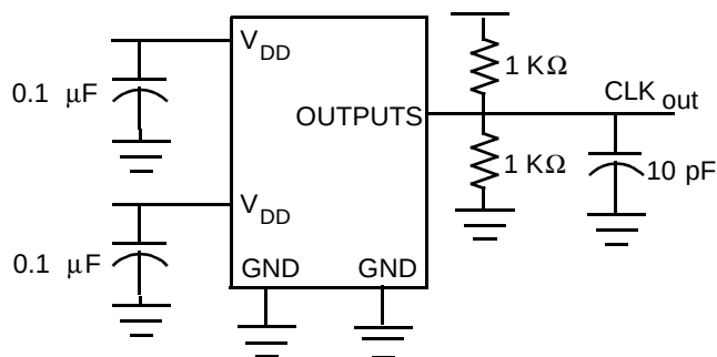
Test Circuit for t_{\phi} , Output slew rate on -1H, -5 device
