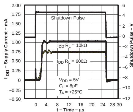
SHUTDOWN PULSE CURRENT vs TIME
