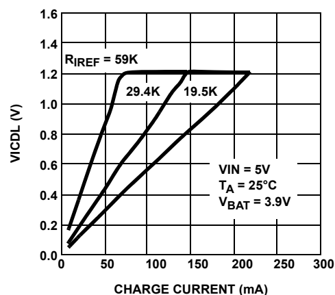
FIGURE 4. VICDL vs CHARGE CURRENT
