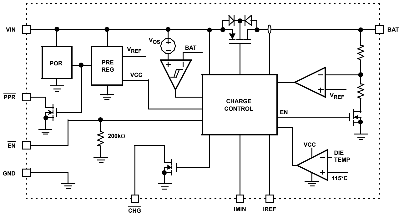
FIGURE 11. BLOCK DIAGRAM
