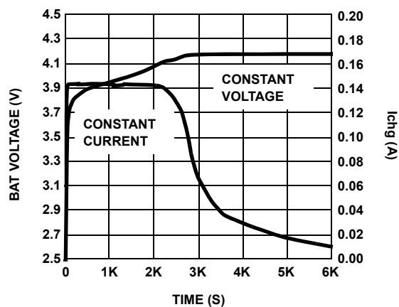
FIGURE 1. COMPLETE CHARGE CYCLE (130mAh BATTERY)
