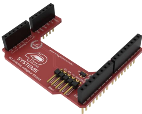
4D Arduino Adaptor Shield
