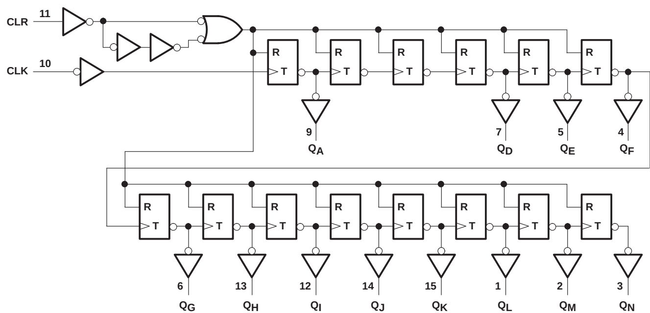
logic diagram (positive logic)
