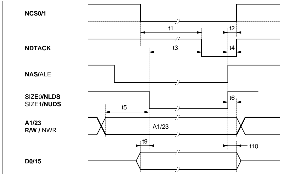
Figure 53 : 68000 Write Cycle
