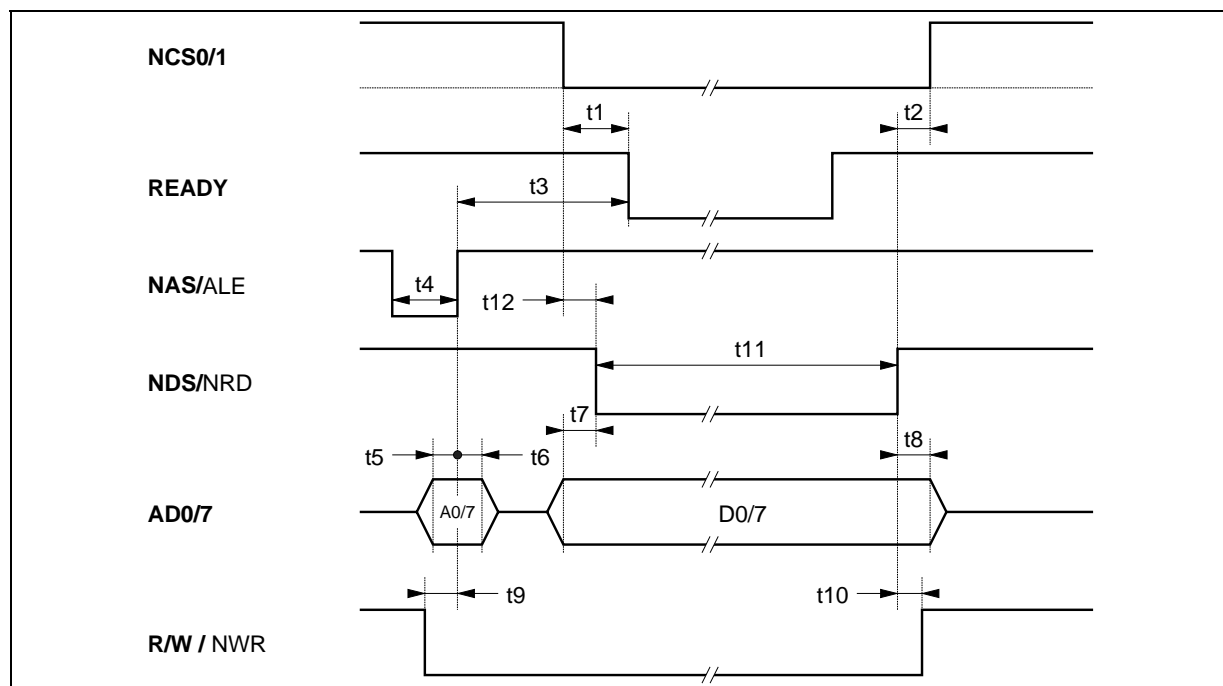
Figure 43 : ST9 Write Cycle
