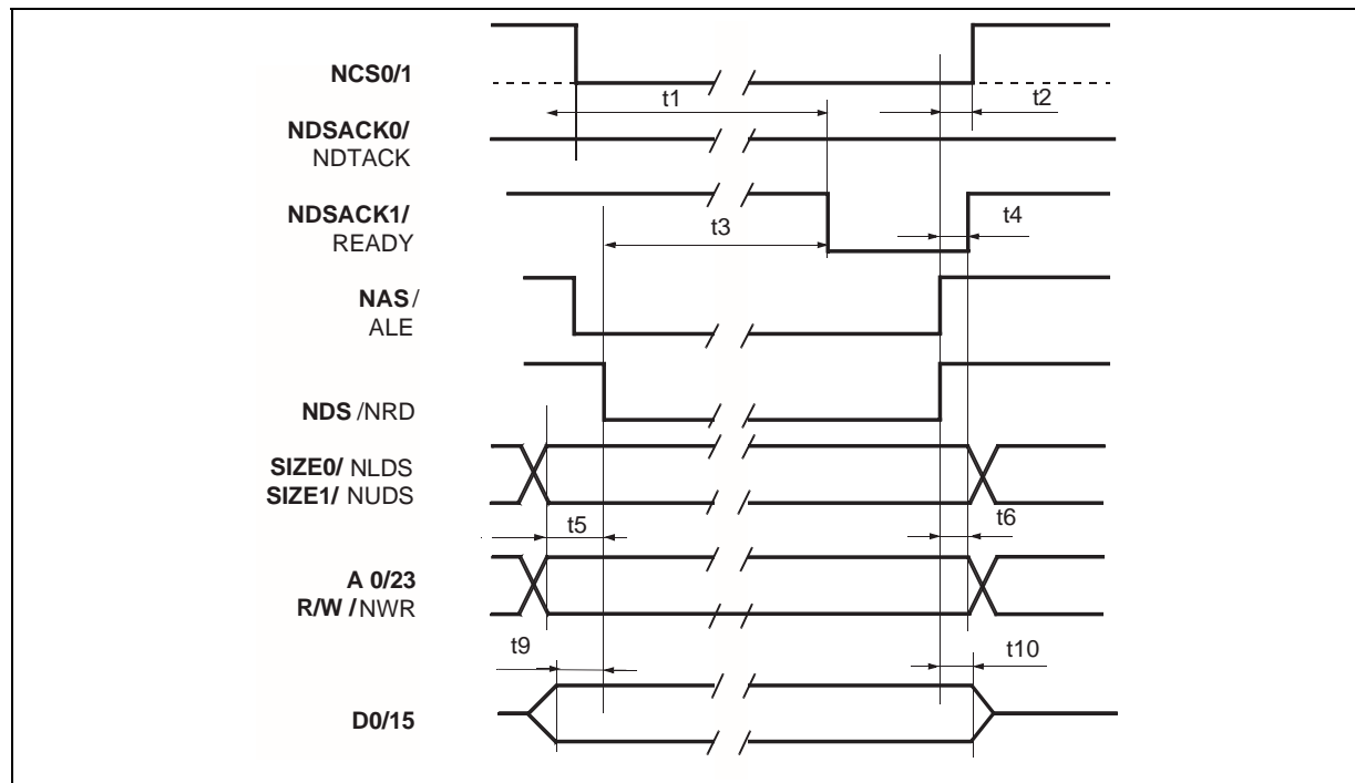
Figure 55 : 68020 Write Cycle
